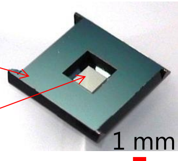
2 mm x 2 mm x 0.2 \mu\text{m} SiC poly-crystal membrane
