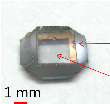
2 mm x 2 mm x 3 \mu\text{m} Quartz membrane
