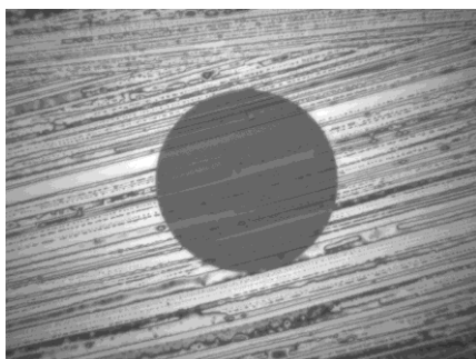
Connector endface before cleaning
